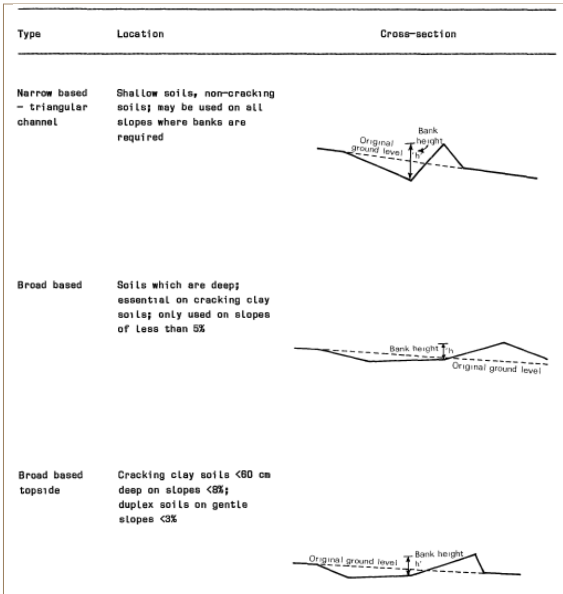
Figure 19. Characteristics of contour bank types used in the Atherton–Mareeba district. From Shepherd RN and Macnish SE (1989). Land Management Field Manual, Atherton–Mareeba District . Queensland Department of Primary Industries, Brisbane.
